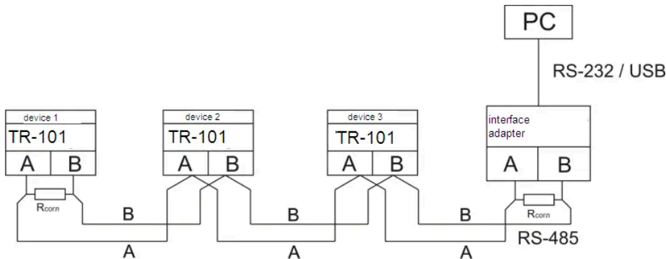
Figure A1 – RS-485 Network Connection Diagram
